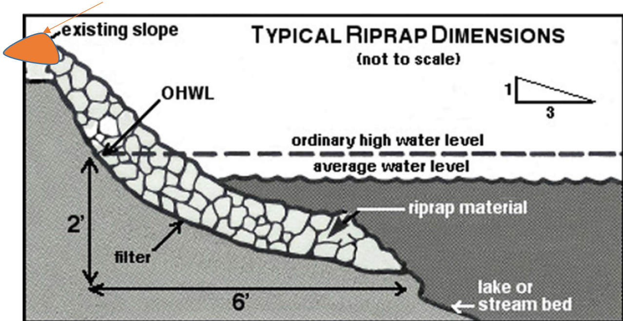
Figure 2-Both cross sections taken from MN DNR Riprap guidelines with Isanti County recommendations.
